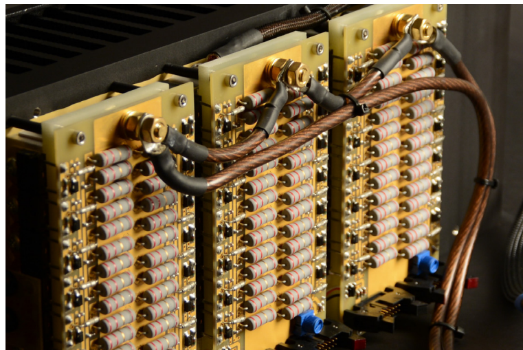
MTP high-current output stage - HQS 9001 mono amplifier
